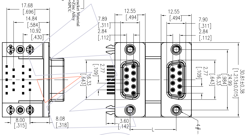
6200-X09FX09FXXX1(WITHOUT SCREW)
